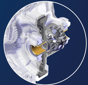
FREE DIFFERENTIAL
